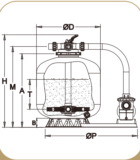
EBF350~EBF700
